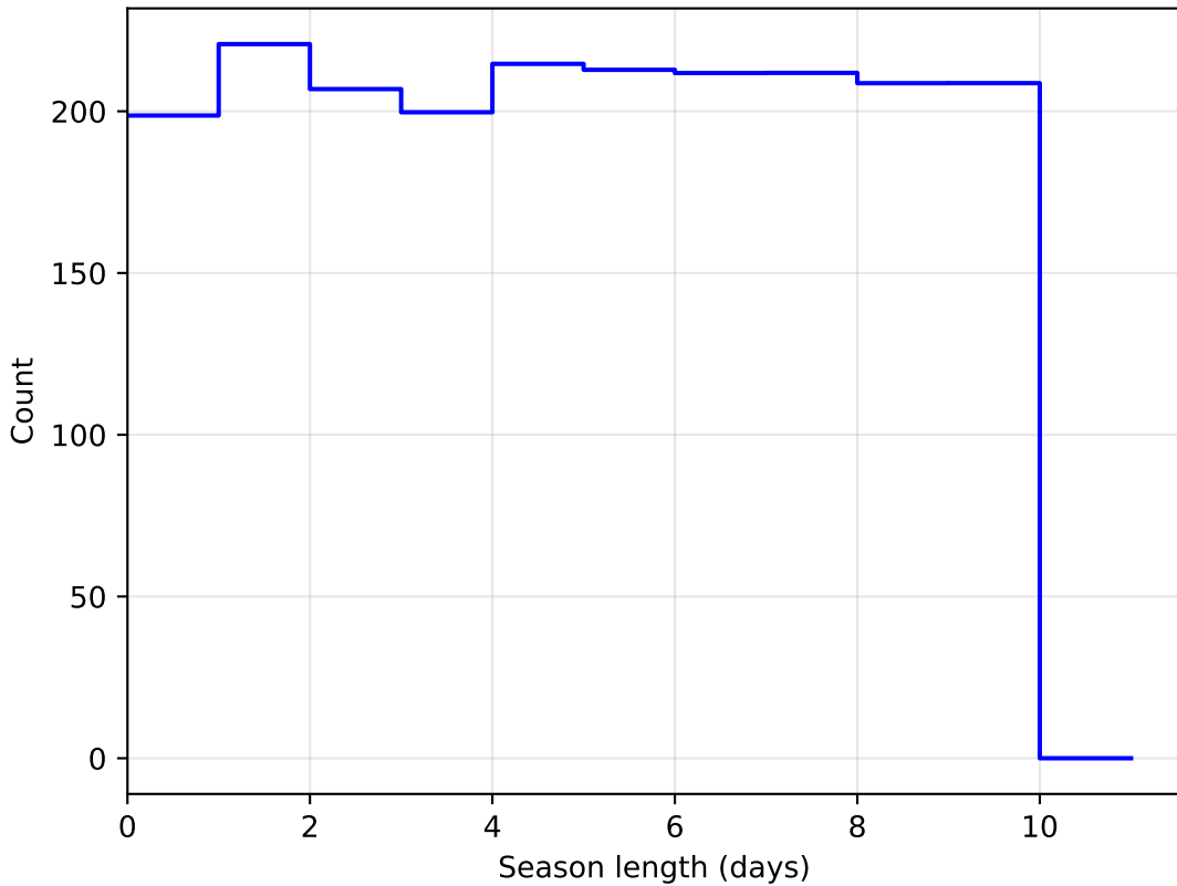
smc_lmc_v3.3_10yrs DD:ELAISS1 all bands: SeasonLength
