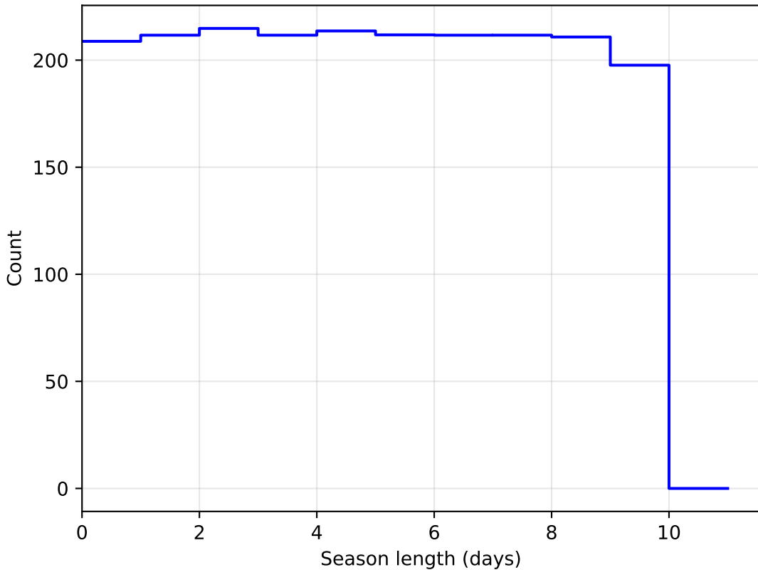
smc_lm_v3.3_10yrs DD:EDFS all bands: SeasonLength
