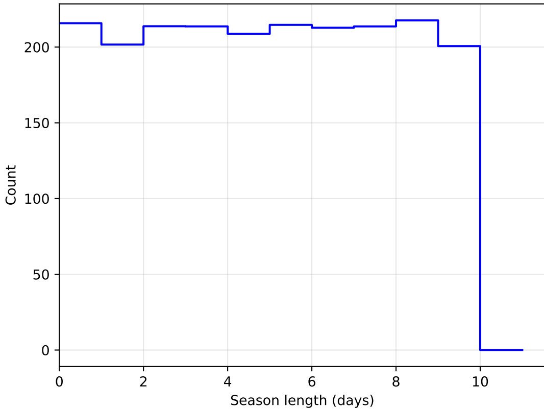
smc_lmc_v3.3_10yrs DD:ECDFS all bands: SeasonLength
