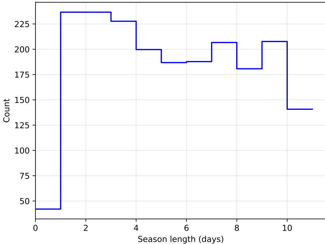
smc_lmc_v3.3_10yrs DD: COSMOS all bands: SeasonLength
