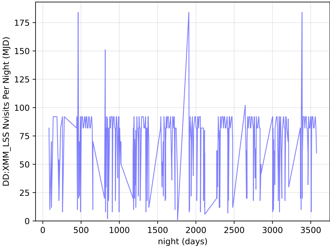
smc_lmc_v3.3_10yrs all bands: DD:XMM_LSS Nvisits Per Night
