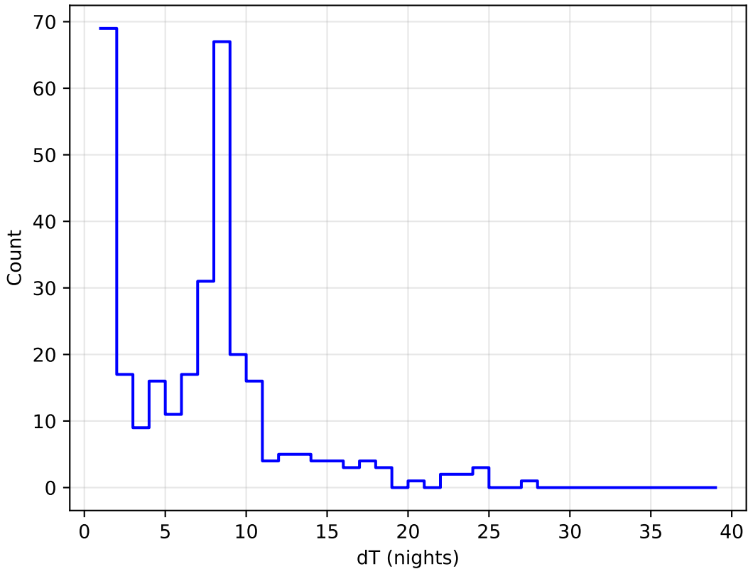
smc_lmc_v3.3_10yrs all bands: DD:XMM_LSS Delta Nights Histogram
