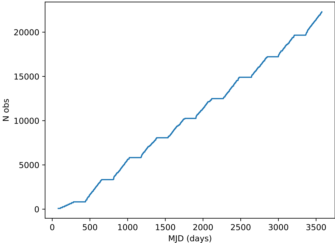
smc_lmc_v3.3_10yrs all bands: DD:XMM_LSS Cumulative NVisits
