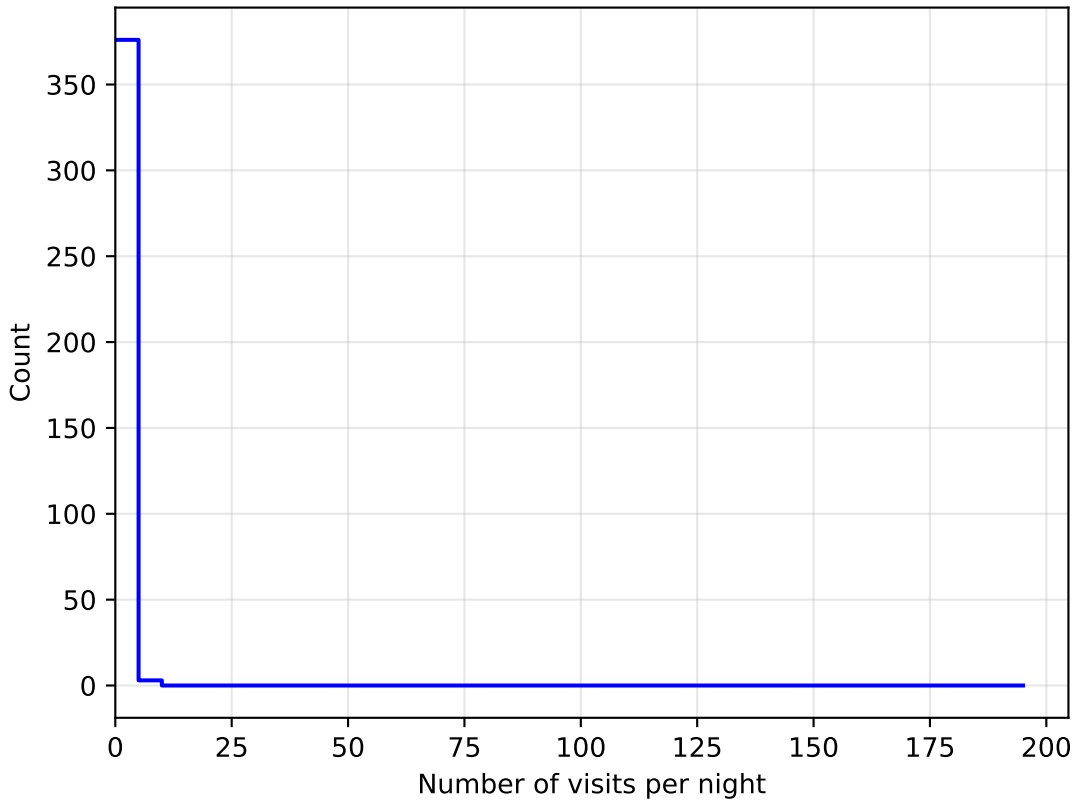
smc_lmc_v3.3_10yrs all bands: DD:WFD NVisitsPerNight
