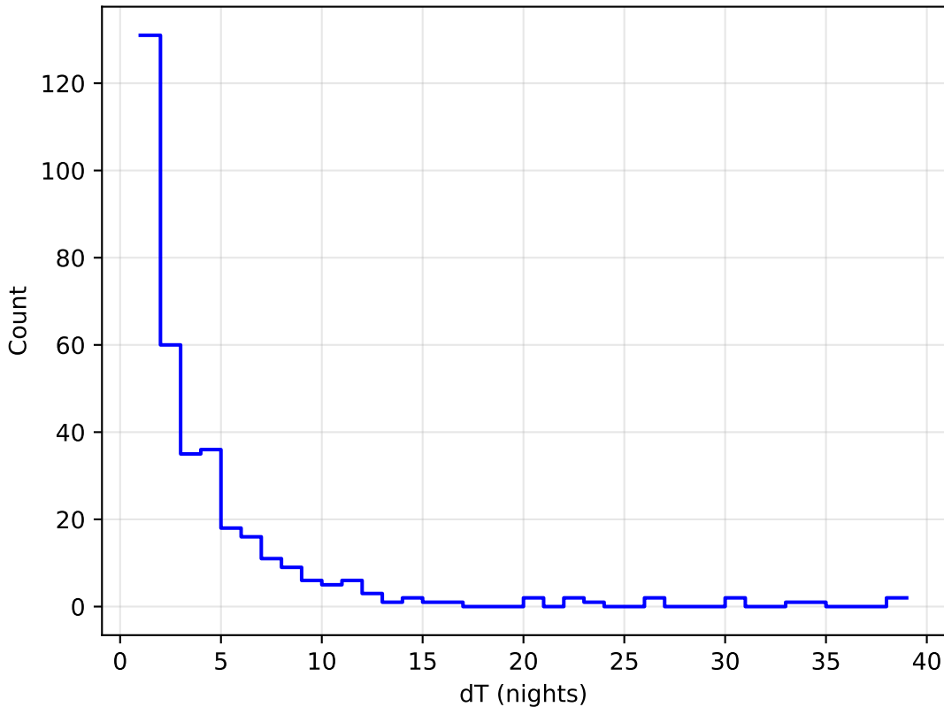
smc_lmc_v3.3_10yrs all bands: DD:WFD Delta Nights Histogram
