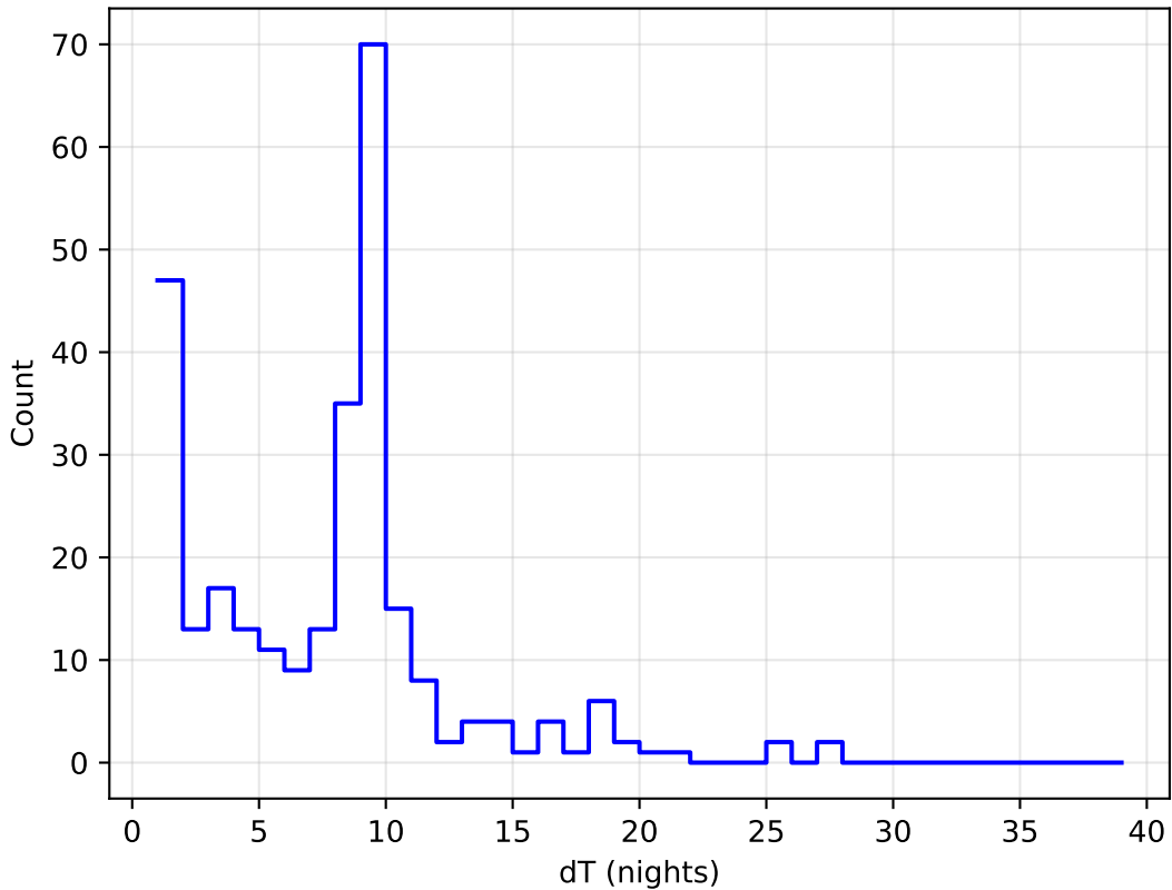
smc_Imc_v3.3_10yrs all bands: DD:ELAISS1 Delta Nights Histogram
