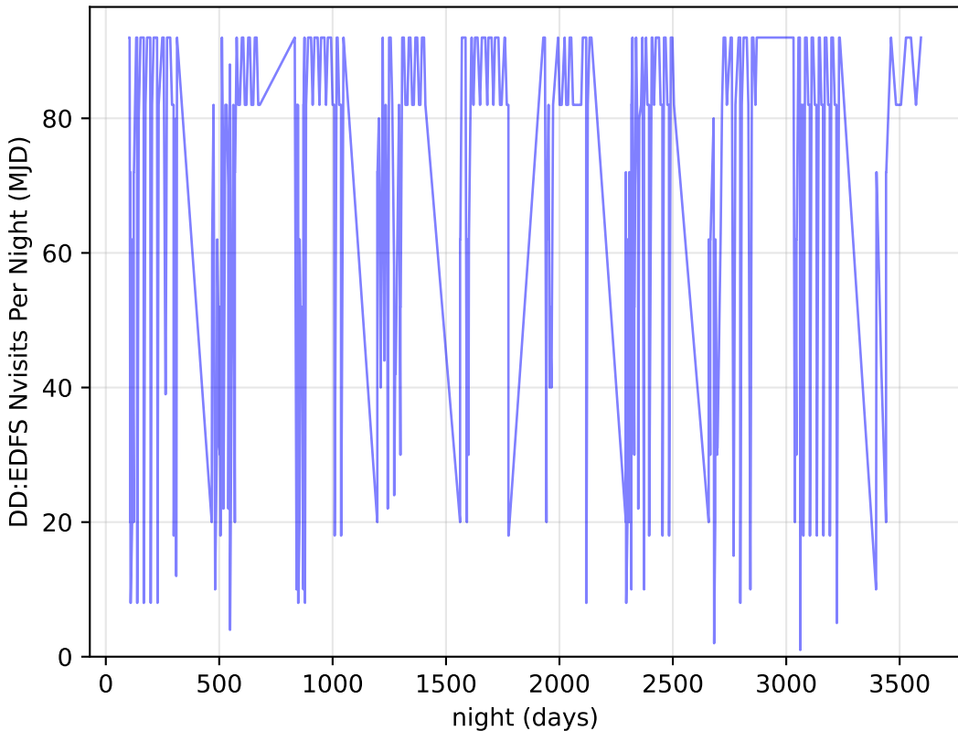
smc_Imc_v3.3_10yrs all bands: DD:EDFS Nvisits Per Night
