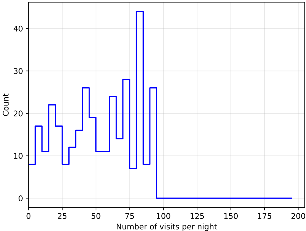
smc_lmc_v3.3_10yrs all bands: DD:EDFS NVisitsPerNight
