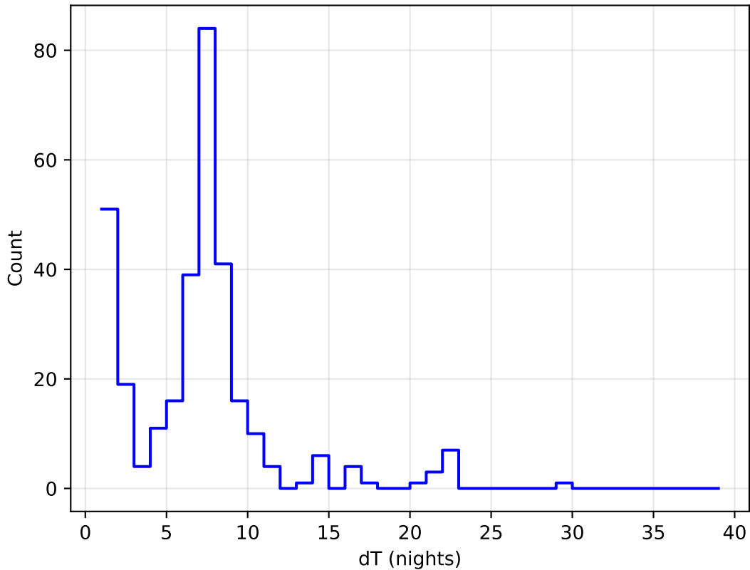
smc_lmc_v3.3_10yrs all bands: DD:EDFS Delta Nights Histogram
