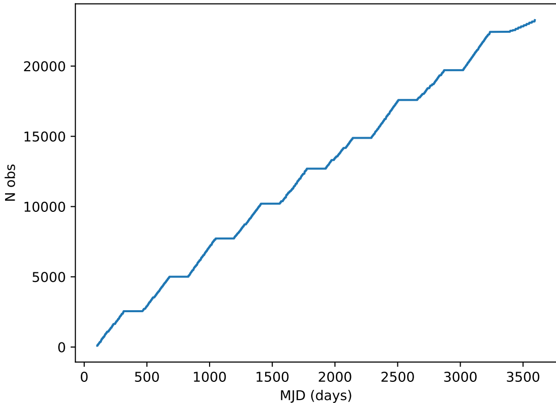
smc_lmc_v3.3_10yrs all bands: DD:EDFS Cumulative NVisits
