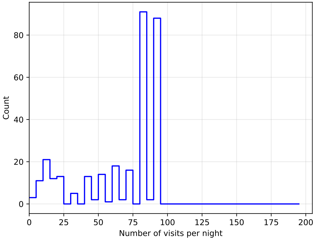
smc_lmc_v3.3_10yrs all bands: DD:ECDFS NVisitsPerNight
