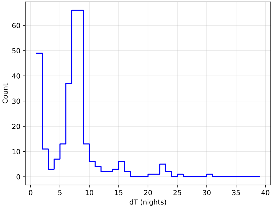
smc_lmc_v3.3_10yrs all bands: DD:ECDFS Delta Nights Histogram
