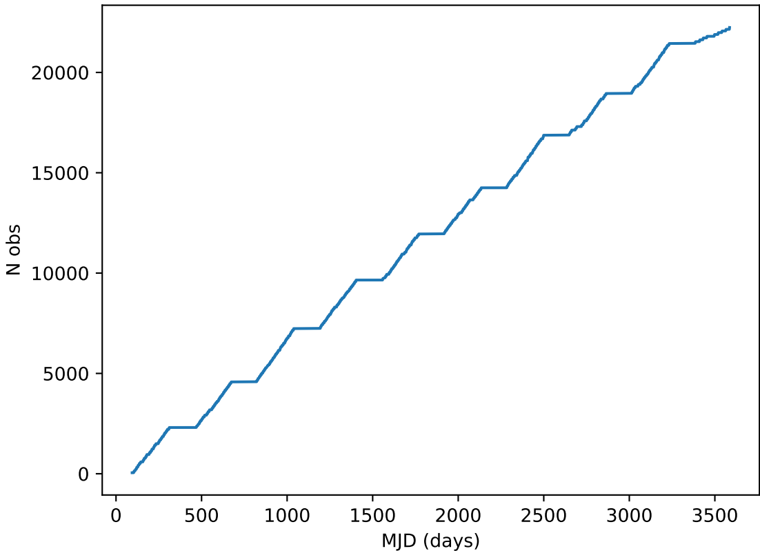
smc_lmc_v3.3_10yrs all bands: DD:ECDFS Cumulative NVisits
