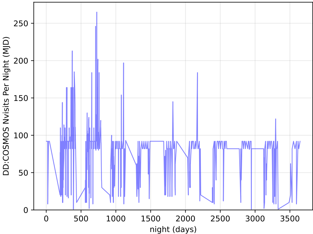
smc_lmc_v3.3_10yrs all bands: DD: COSMOS Nvisits Per Night
