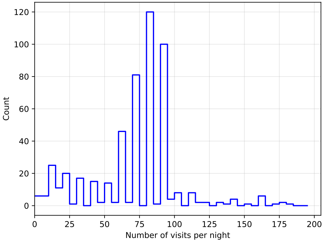
smc_lmc_v3.3_10yrs all bands: DD: COSMOS NVisitsPerNight
