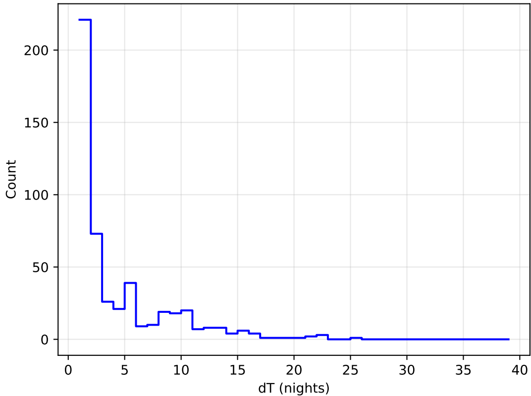
smc_Imc_v3.3_10yrs all bands: DD: COSMOS Delta Nights Histogram
