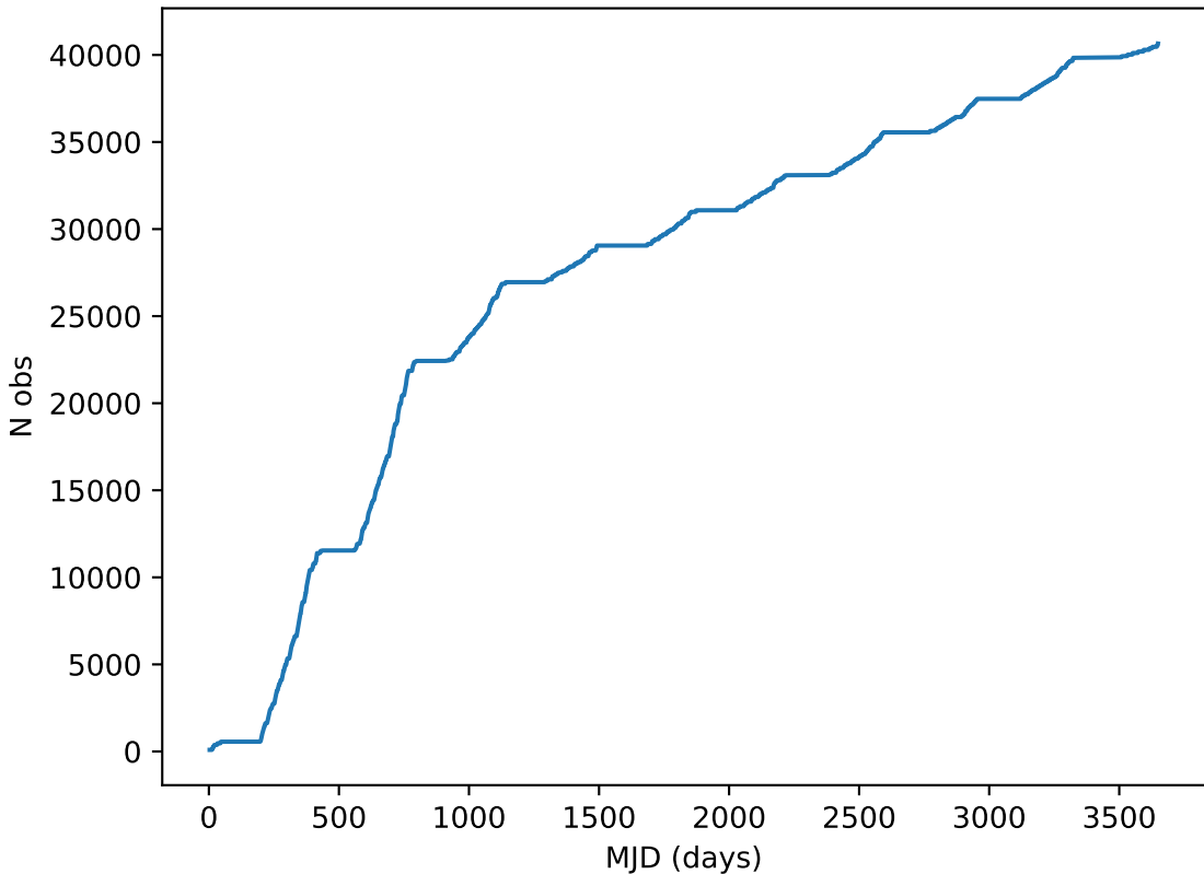
smc_lmc_v3.3_10yrs all bands: DD: COSMOS Cumulative NVisits
