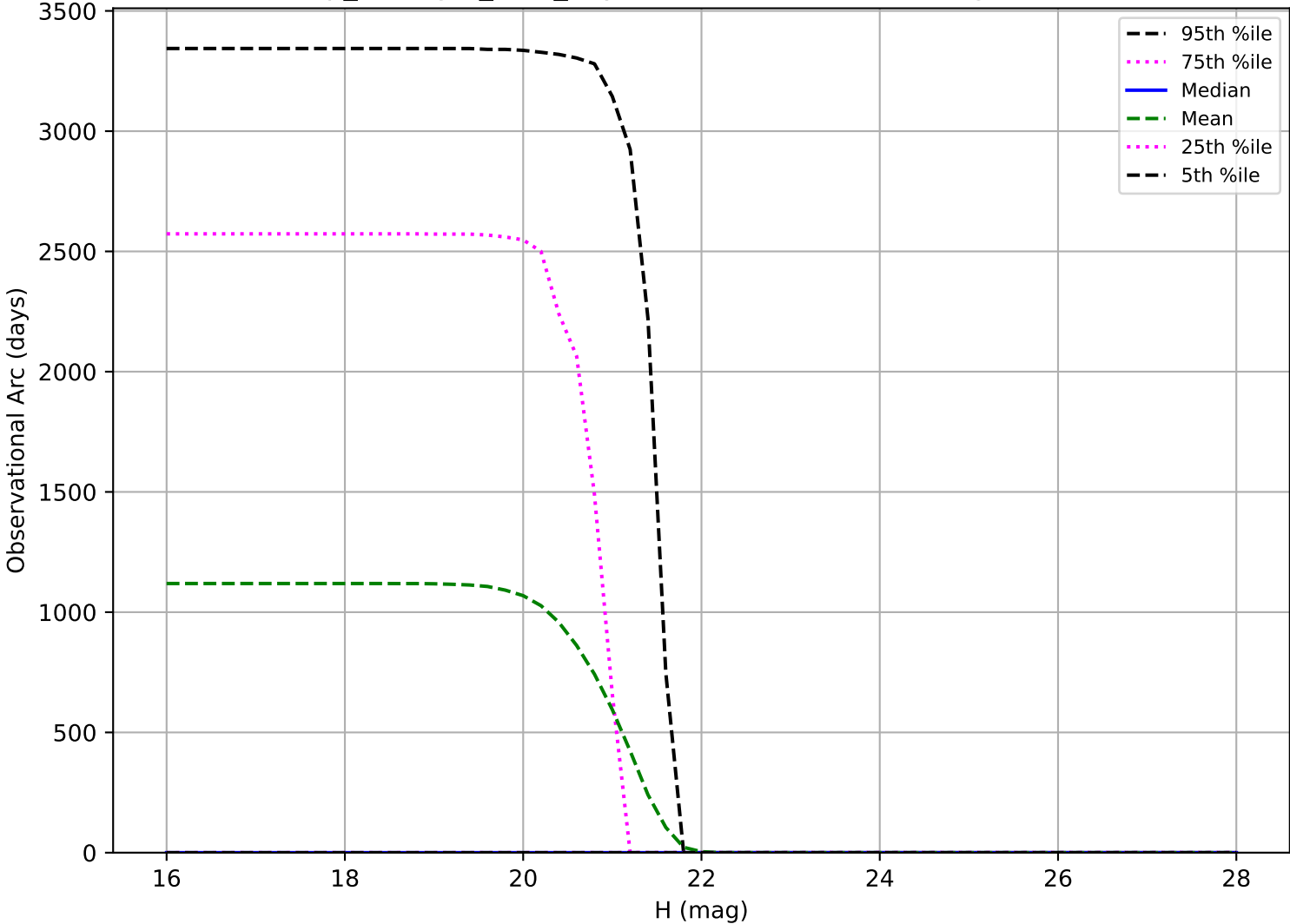
scp_reweight_v3.3_10yrs: Observational Arc Length Vatira
