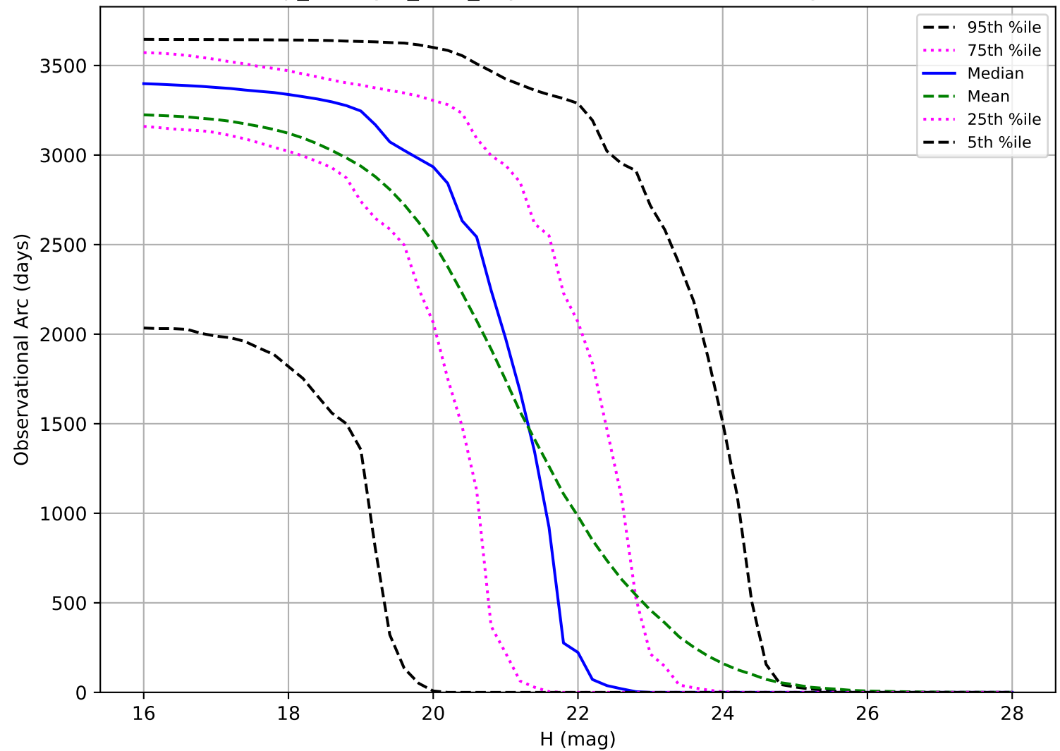
scp_reweight_v3.3_10yrs: Observational Arc Length PHA
