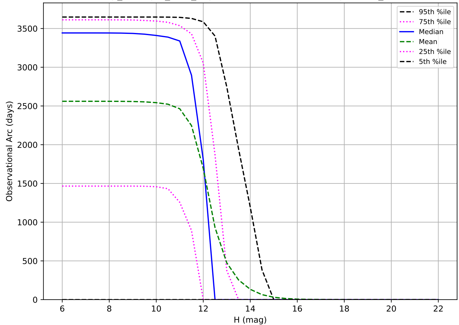
scp_reweight_v3.3_10yrs: Observational Arc Length OCC_r20
