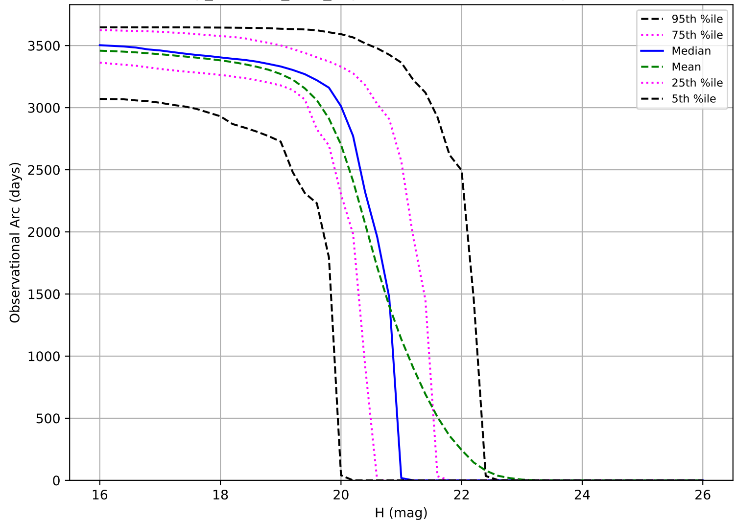
scp_reweight_v3.3_10yrs: Observational Arc Length MBA
