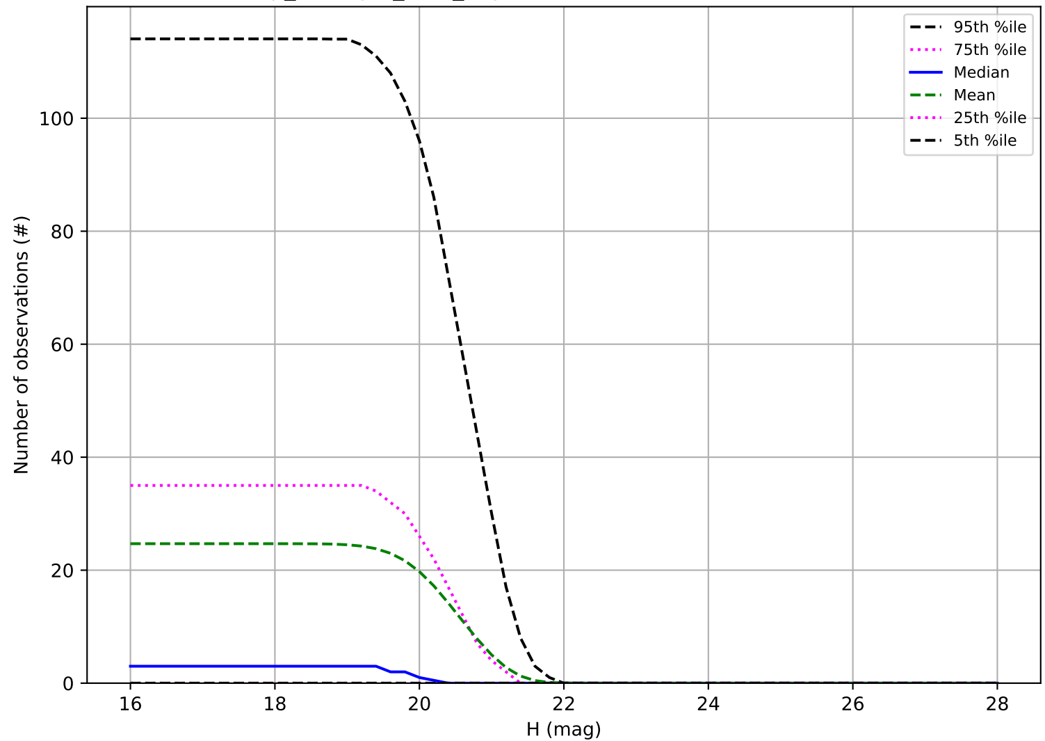
scp_reweight_v3.3_10yrs: Number of observations Vatira
