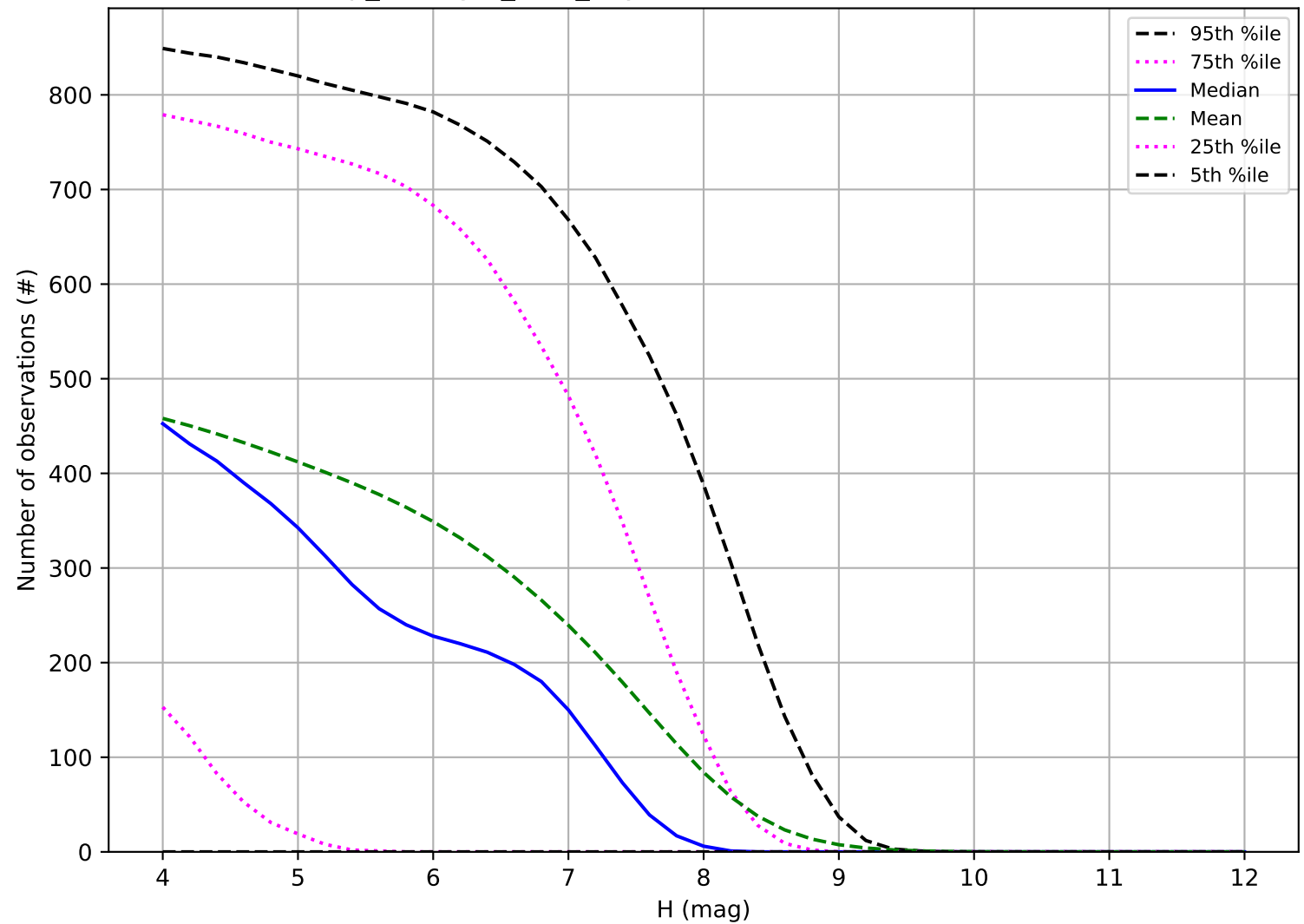
scp_reweight_v3.3_10yrs: Number of observations TNO
