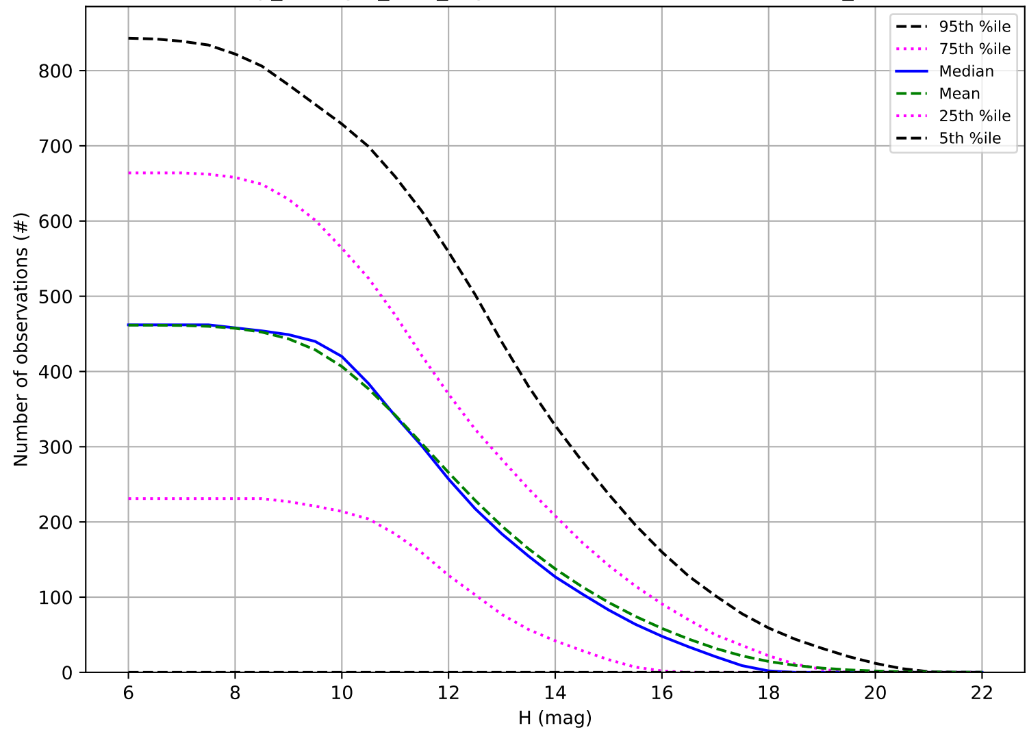
scp_reweight_v3.3_10yrs: Number of observations OCC_r5
