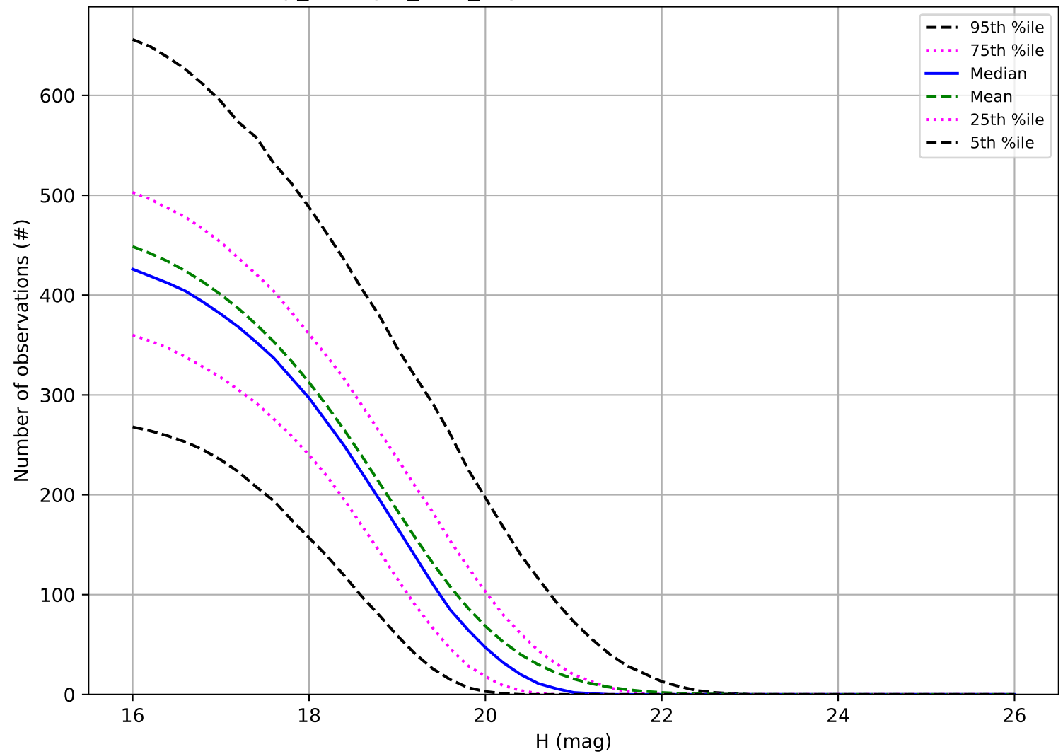
scp_reweight_v3.3_10yrs: Number of observations MBA
