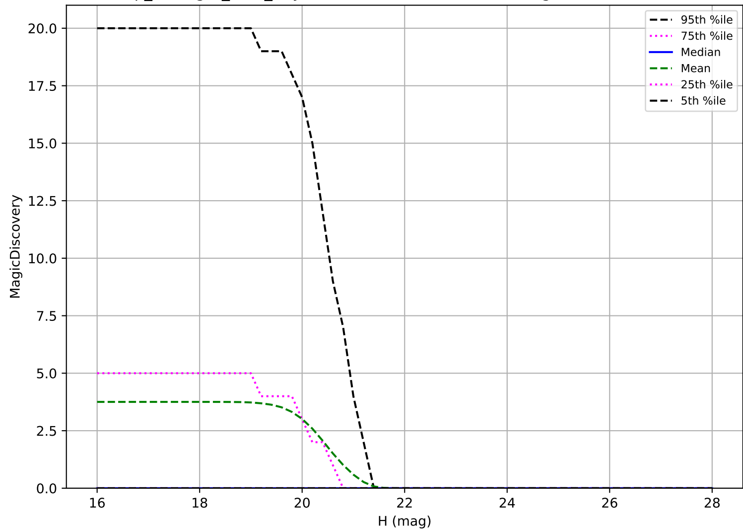
scp_reweight_v3.3_10yrs: Vatira 6 detections in 60 nights detection loss
