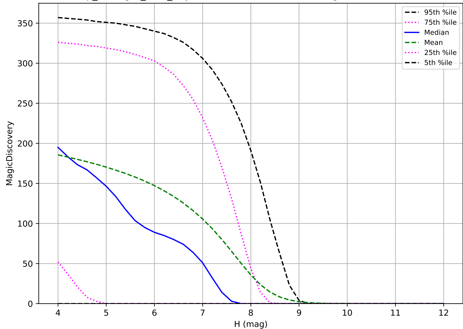
scp_reweight_v3.3_10yrs: TNO 6 detections in 60 nights detection loss
