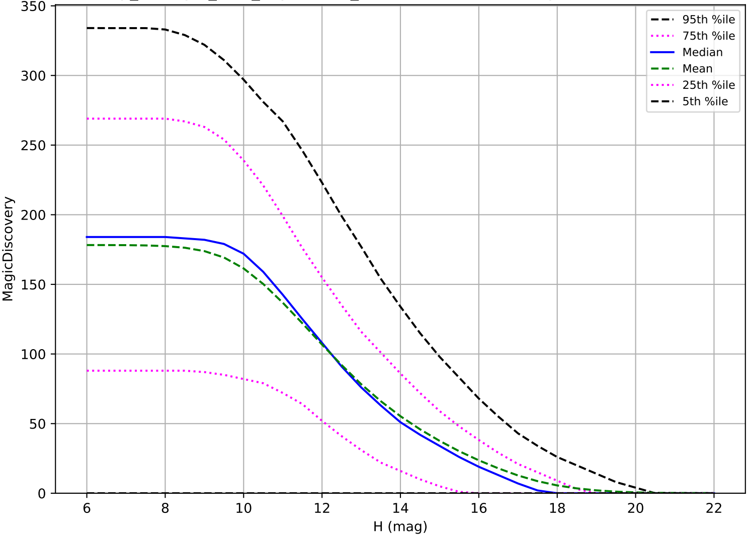
scp_reweight_v3.3_10yrs: OCC_r5 6 detections in 60 nights detection loss
