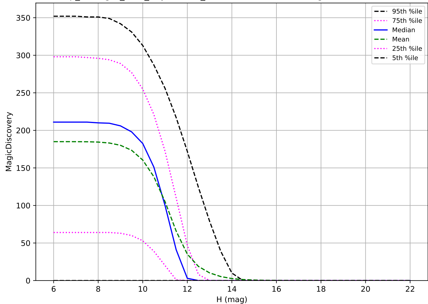
scp_reweight_v3.3_10yrs: OCC_r20 6 detections in 60 nights detection loss
