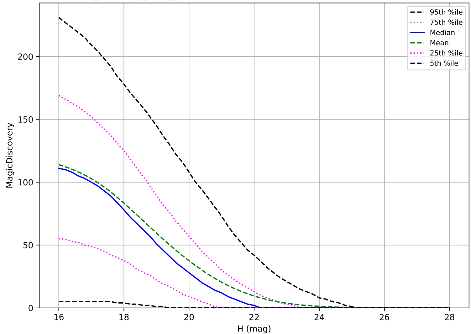
scp_reweight_v3.3_10yrs: NEO 6 detections in 60 nights detection loss
