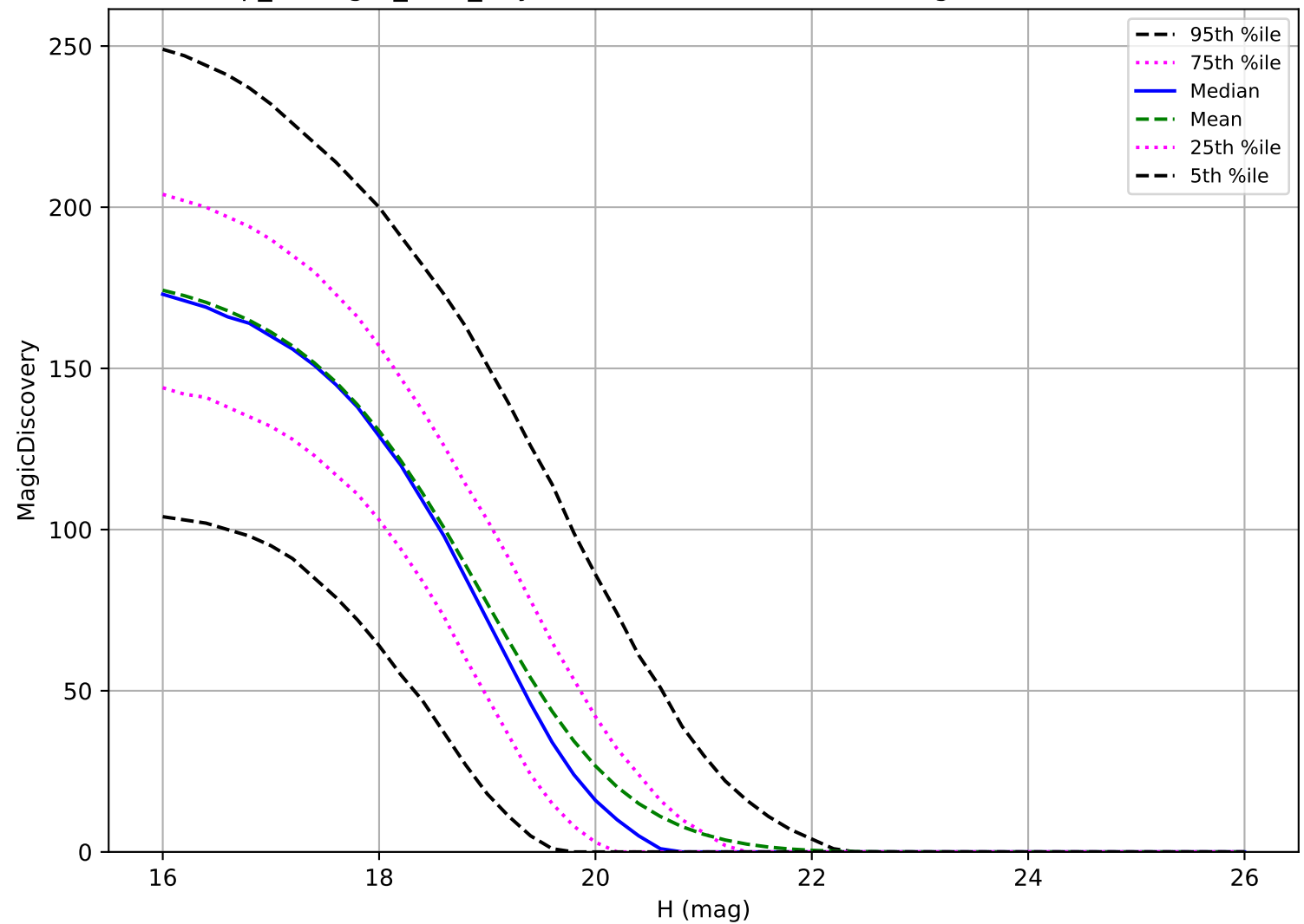
scp_reweight_v3.3_10yrs: MBA 6 detections in 60 nights detection loss
