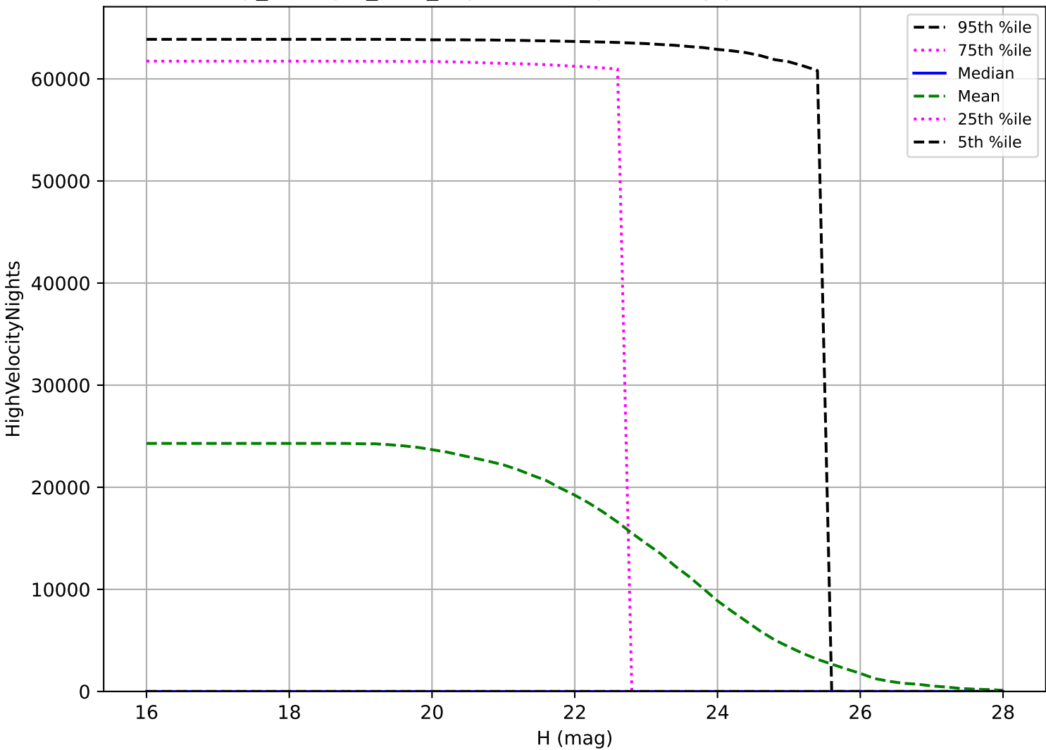
scp_reweight_v3.3_10yrs: PHA High velocity pair detection loss
