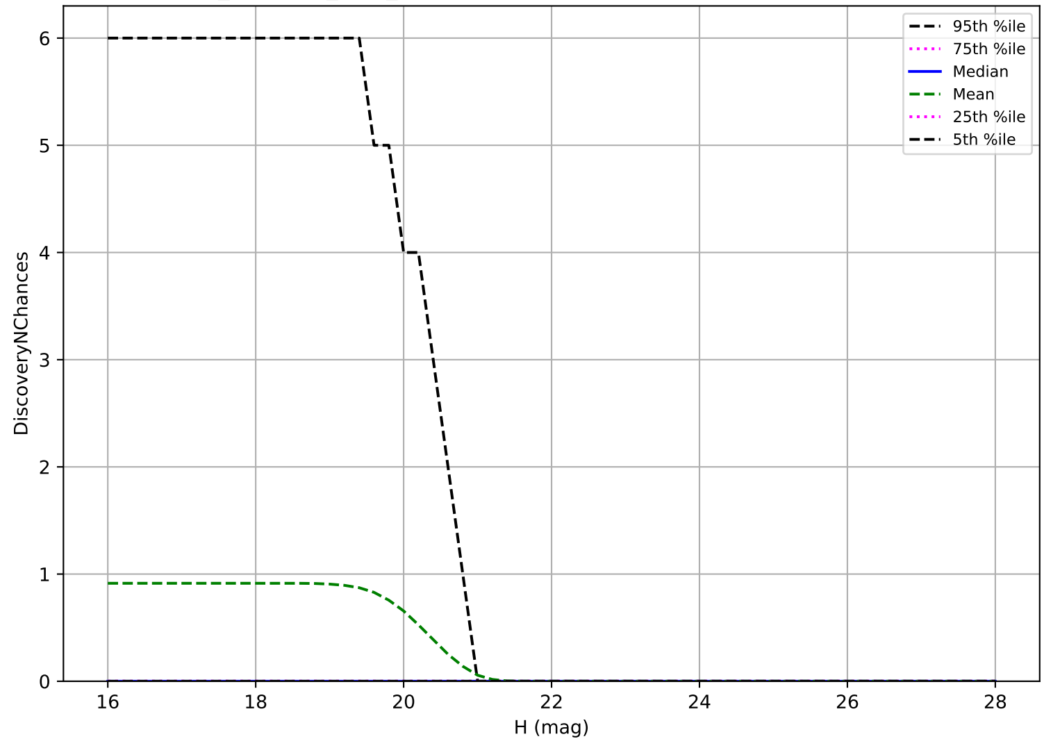
scp_reweight_v3.3_10yrs: Vatira 3 pairs in 15 nights detection loss
