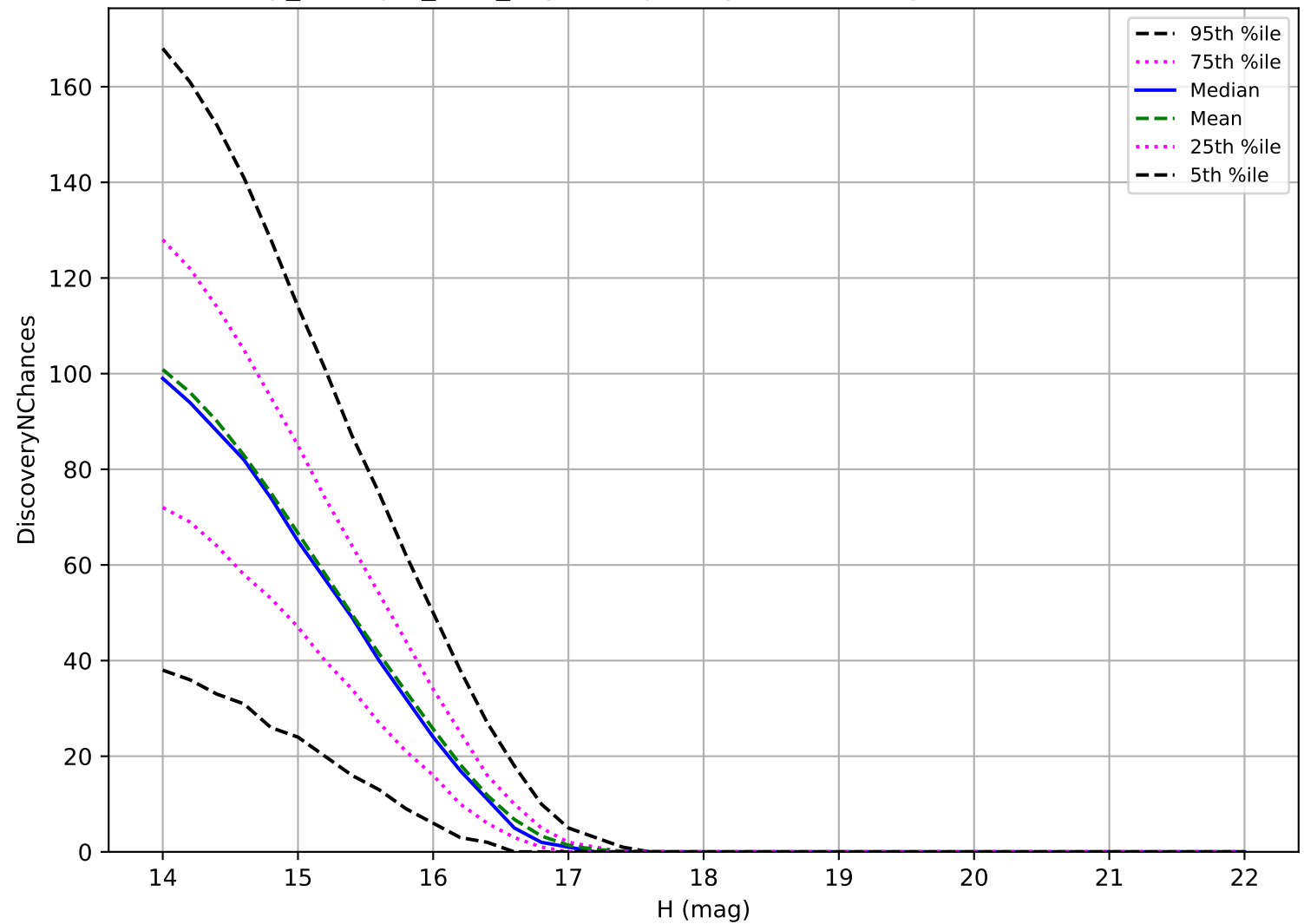
scp_reweight_v3.3_10yrs: Trojan 3 pairs in 15 nights detection loss
