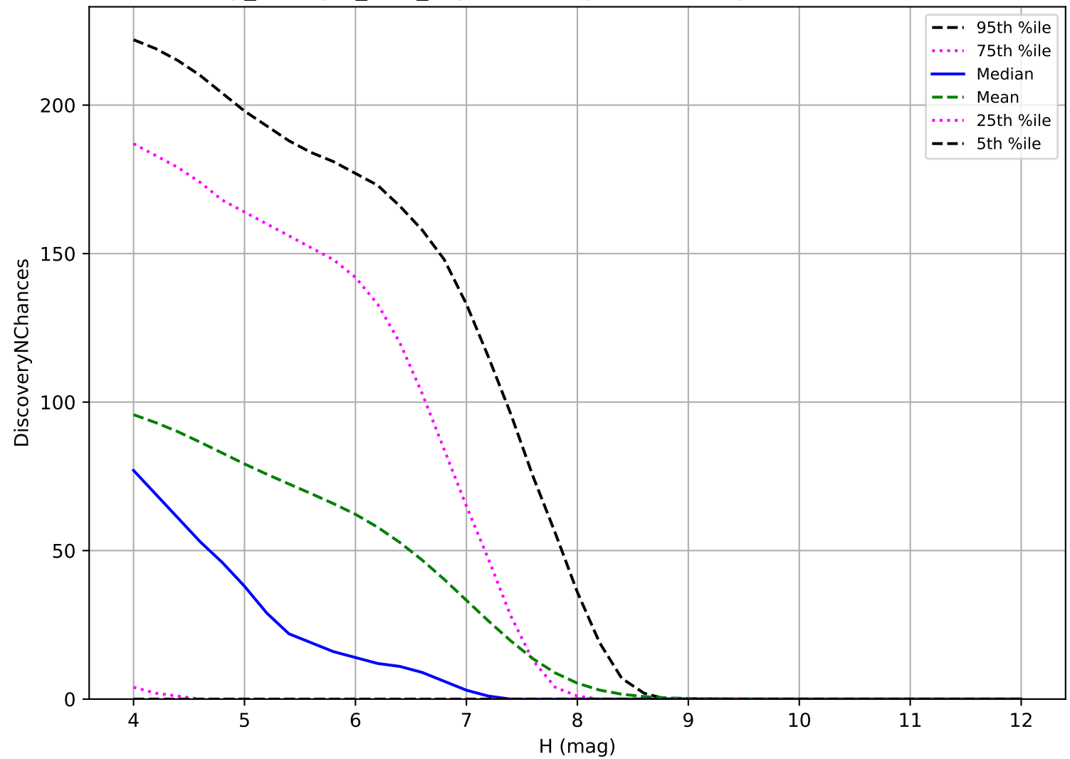
scp_reweight_v3.3_10yrs: TNO 3 pairs in 15 nights detection loss
