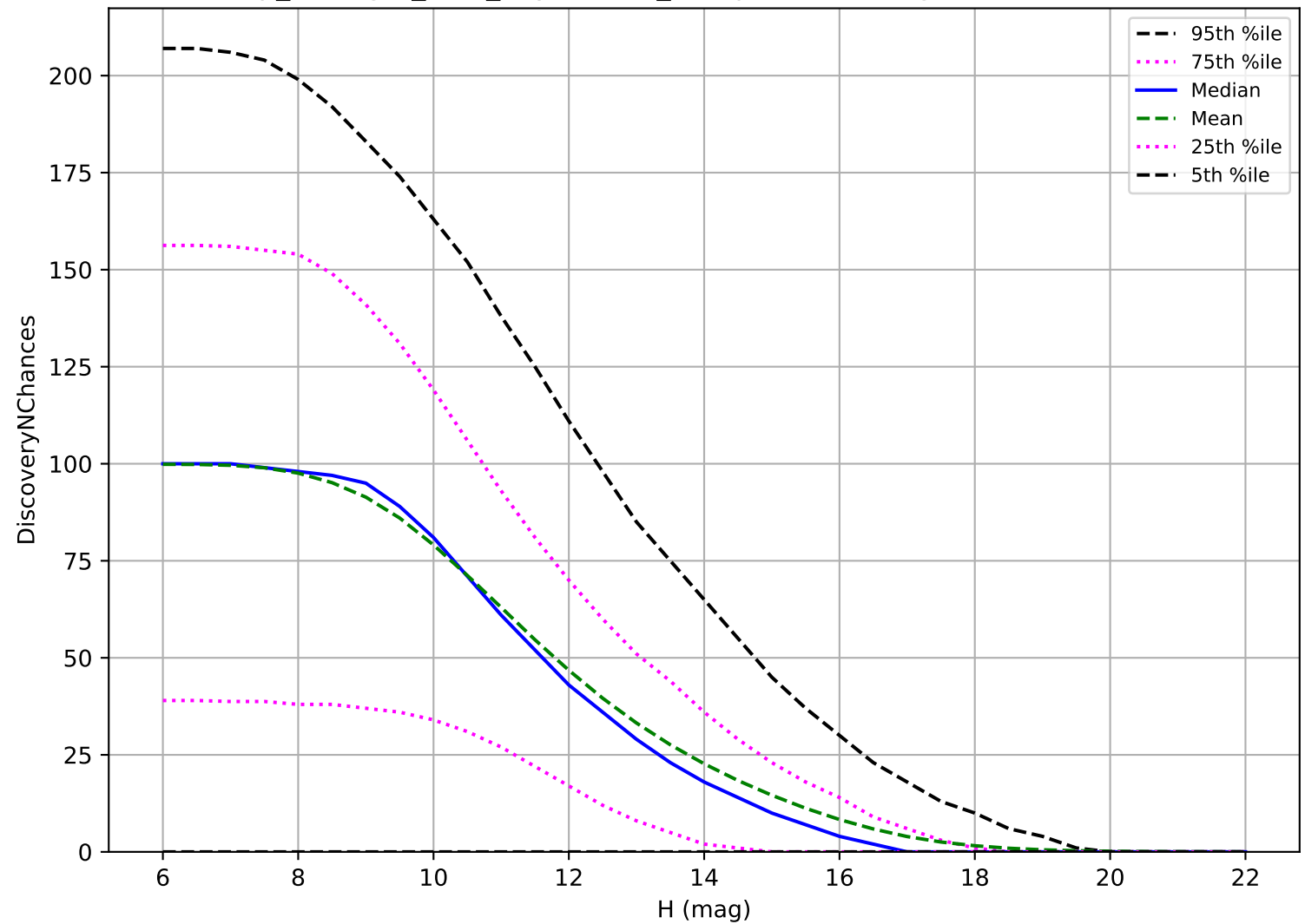
scp_reweight_v3.3_10yrs: OCC_r5 3 pairs in 15 nights detection loss
