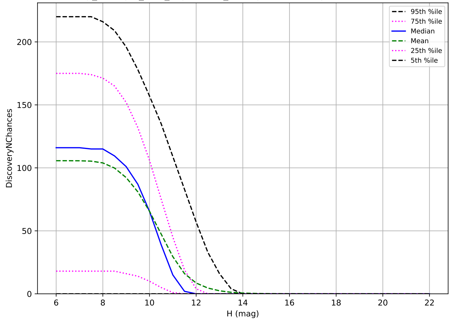
scp_reweight_v3.3_10yrs: OCC_r20 3 pairs in 15 nights detection loss
