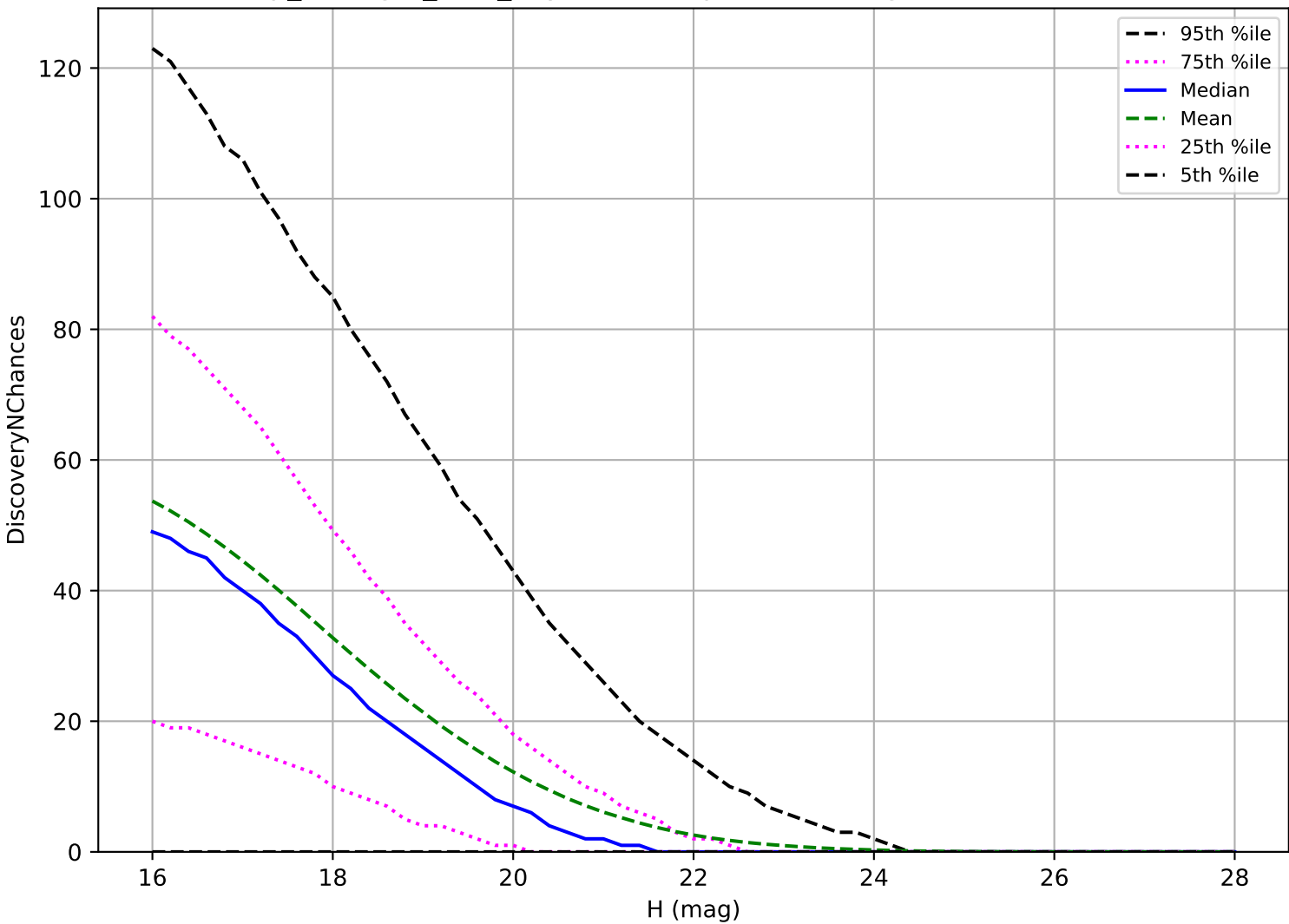
scp_reweight_v3.3_10yrs: NEO 3 pairs in 15 nights detection loss
