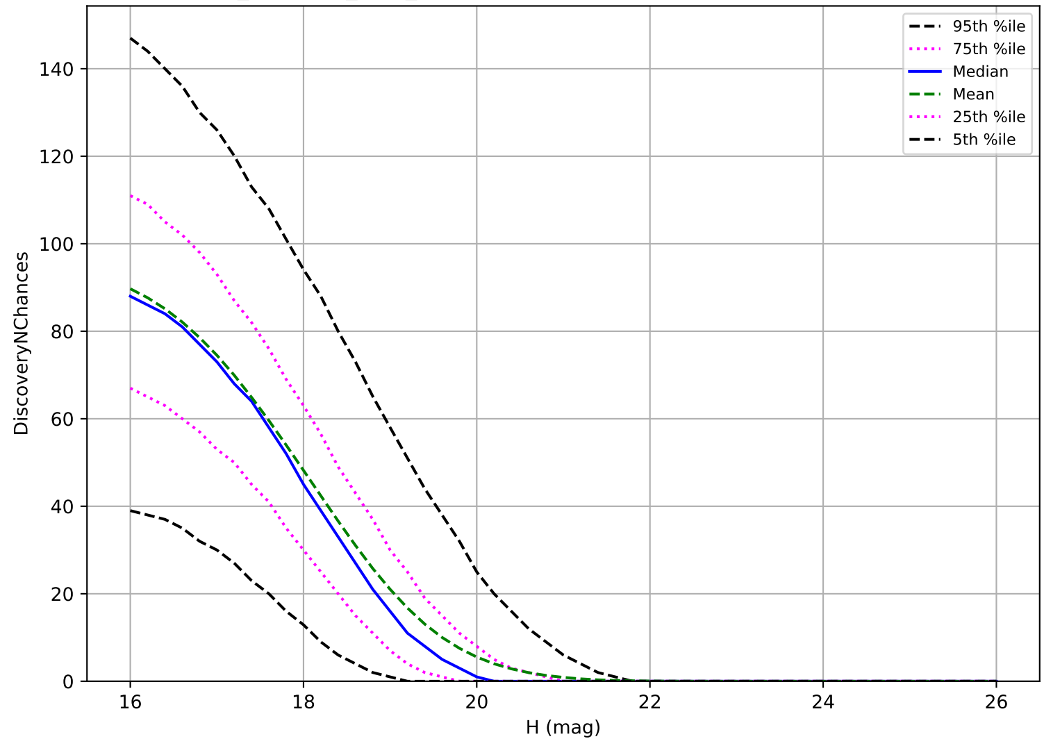
scp_reweight_v3.3_10yrs: MBA 3 pairs in 15 nights detection loss
