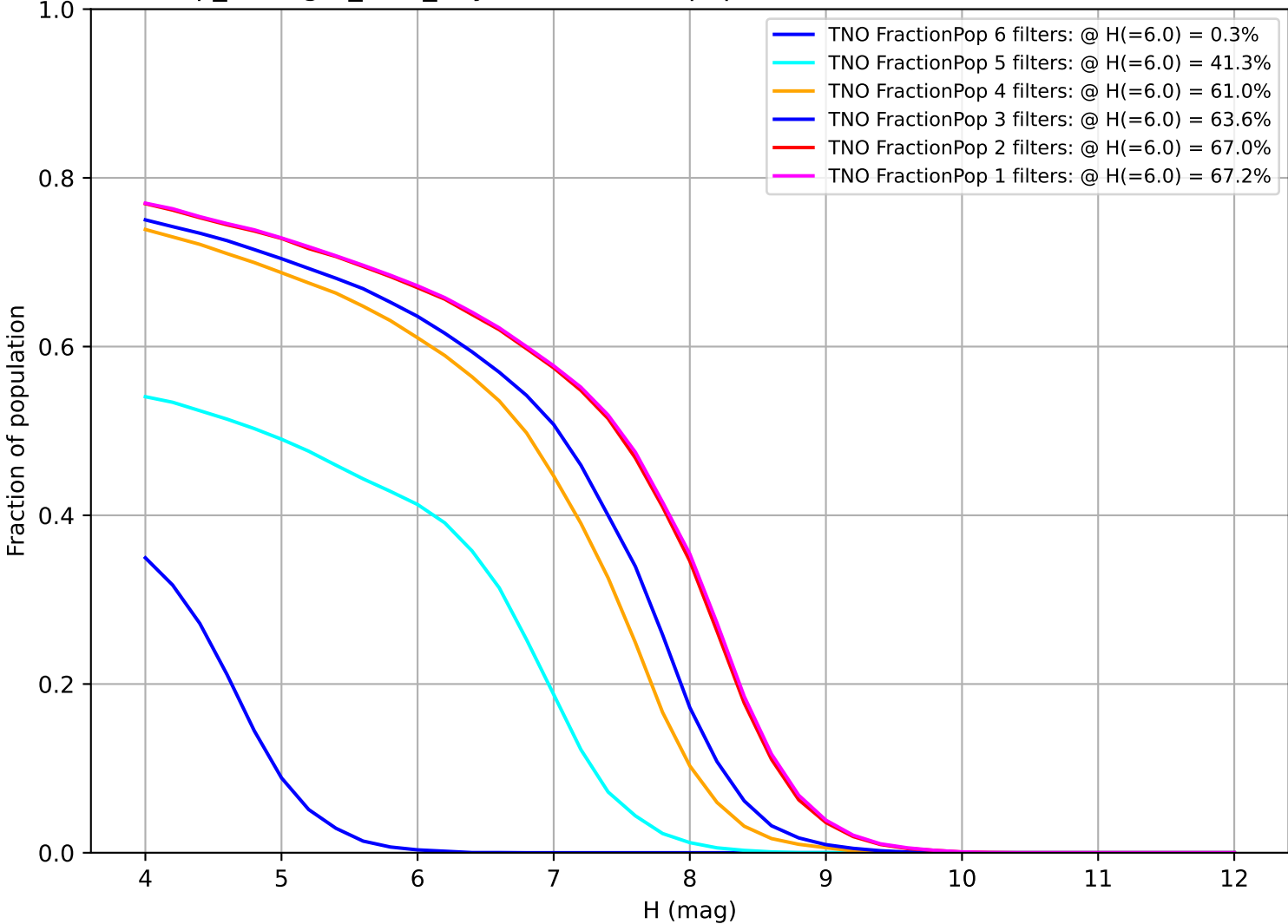
scp_reweight_v3.3_10yrs: Fraction of population with colors in X filters TNO
