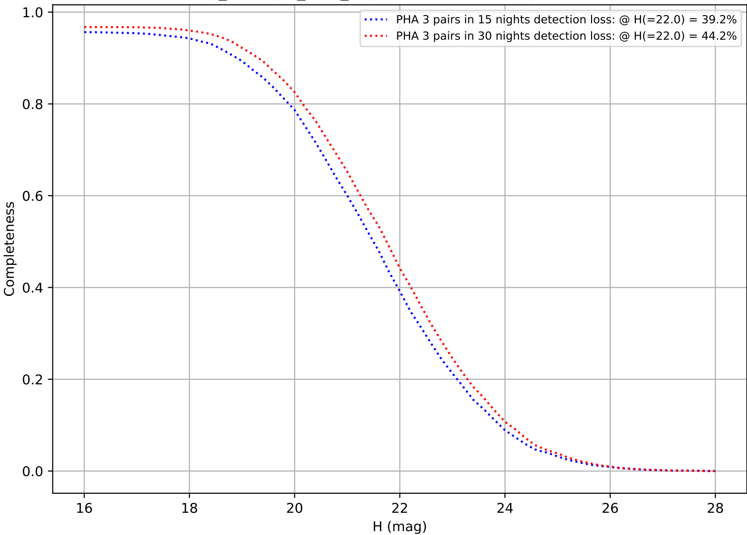
scp_reweight_v3.3_10yrs: DifferentialCompleteness
