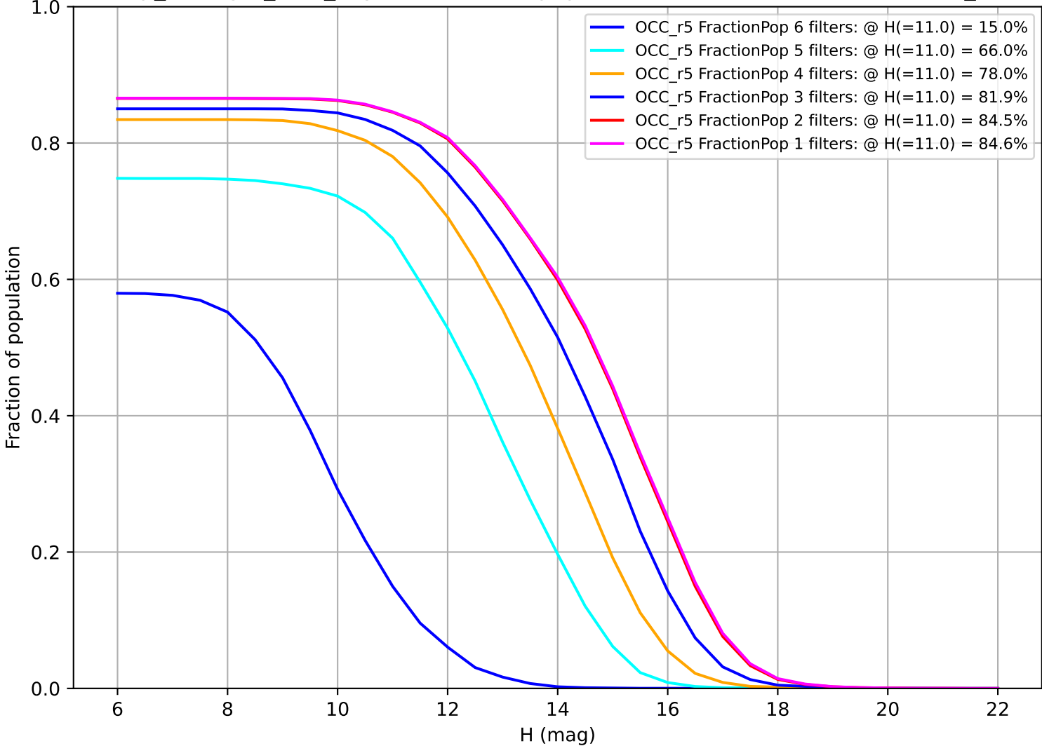
scp_reweight_v3.3_10yrs: Fraction of population with colors in X filters OCC_r5
