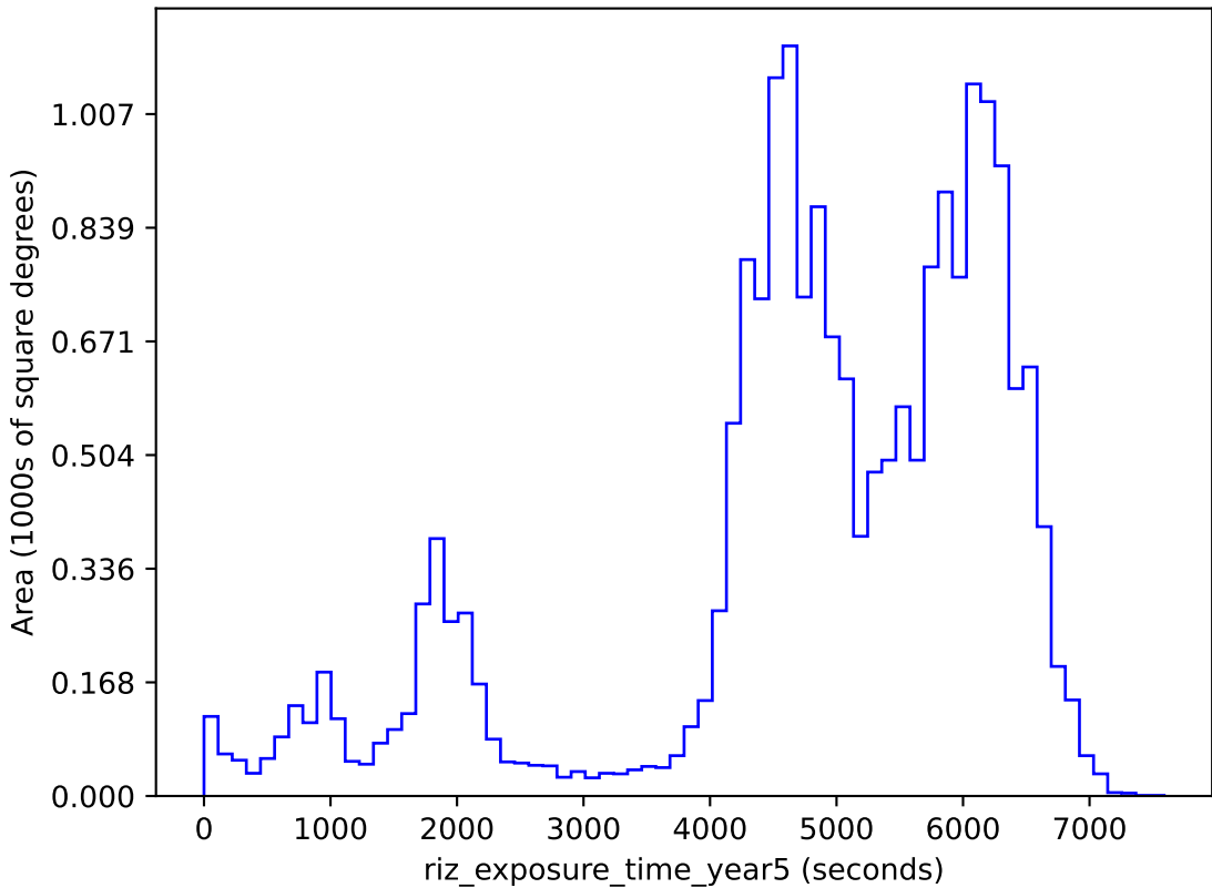
scp_reweight_v3.3_10yrs gri band non-DD: riz_exposure_time_year5
