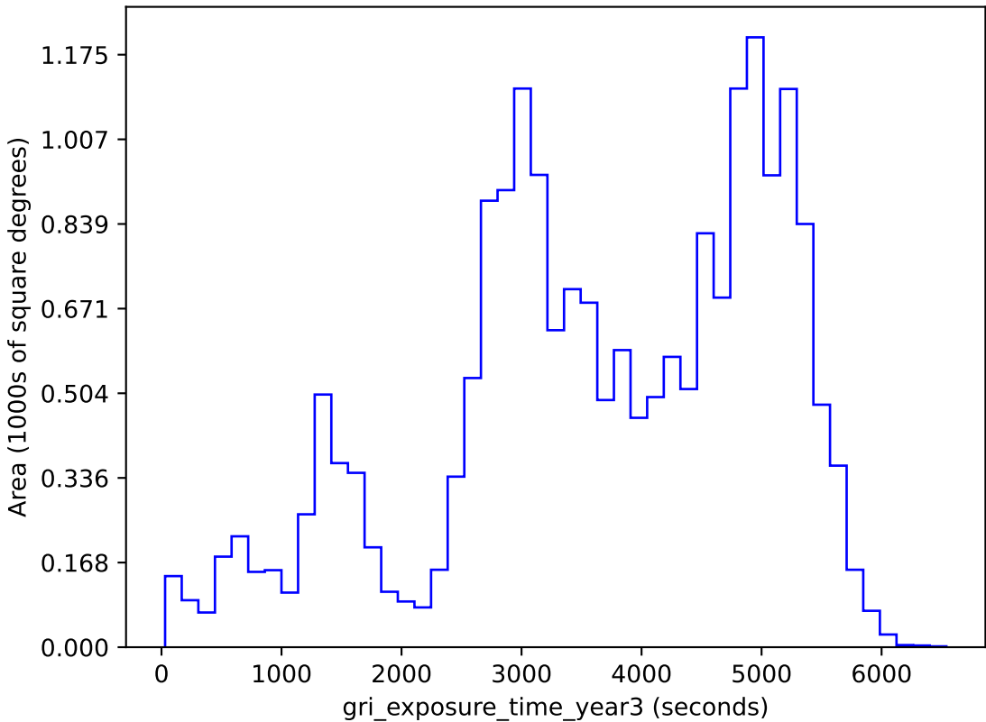
scp_reweight_v3.3_10yrs gri band non-DD: gri_exposure_time_year3
