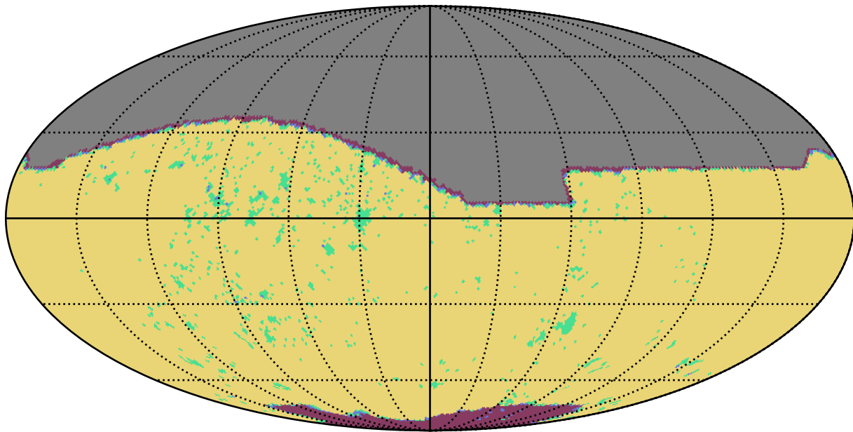
scp_reweight_v3.3_10yrs z band: YearCoverage night
