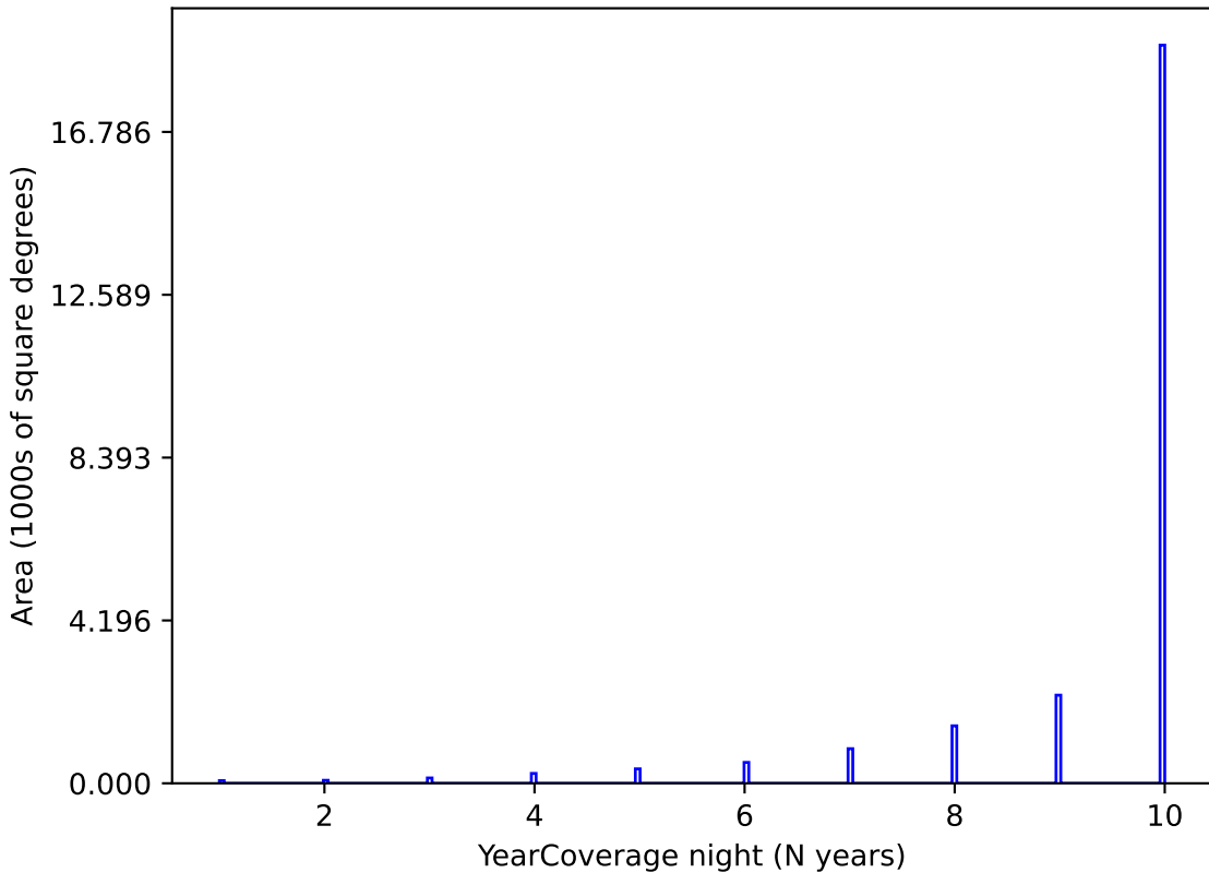
scp_reweight_v3.3_10yrs y band: YearCoverage night
